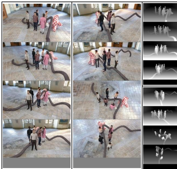
Figure 3. Atlases for Group sequence, MIV View (V17). From left: atlas T0, T1, G0 (top), and G1.
