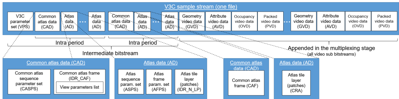
Figure 33: V3C sample stream with MIV extensions
