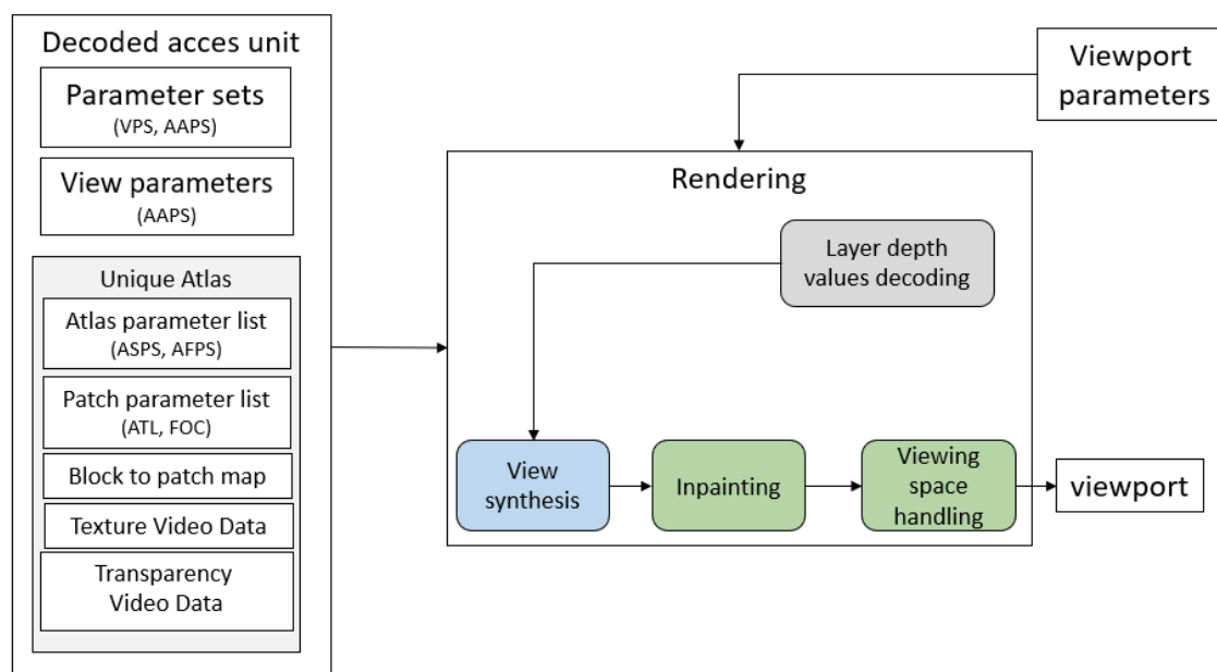
Figure 42: Process flow for TMIV MPI renderer
