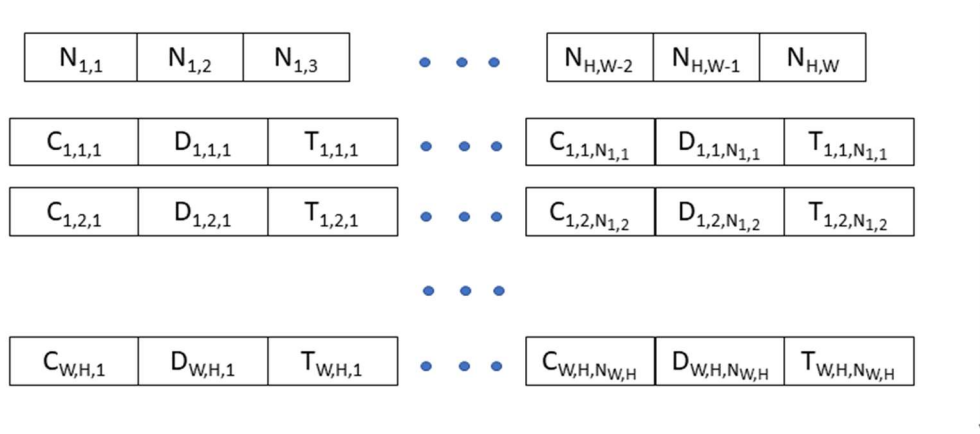
Figure 33: MPI packed compressed storage (PCS) layout.
