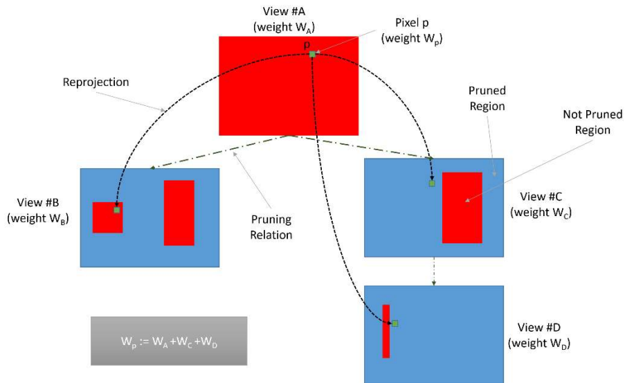
Figure 40: graph-based pruning: weight recovery procedure
