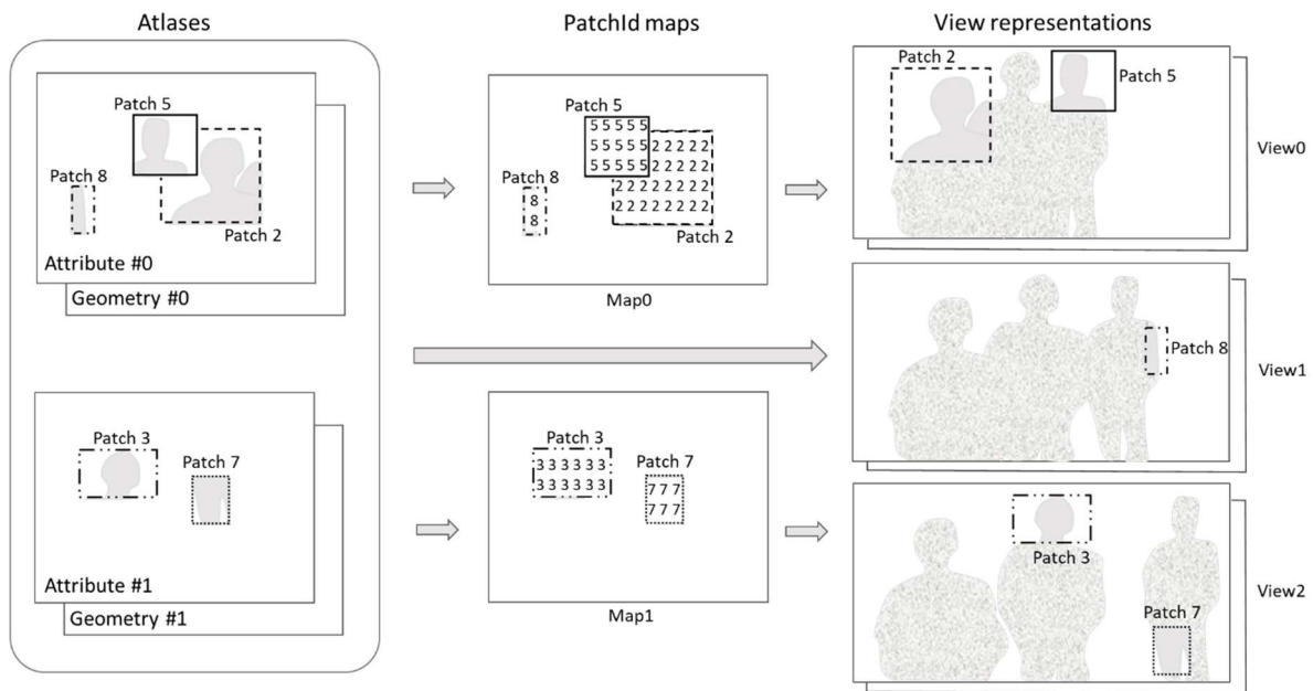
Figure 38: Pruned view reconstruction
