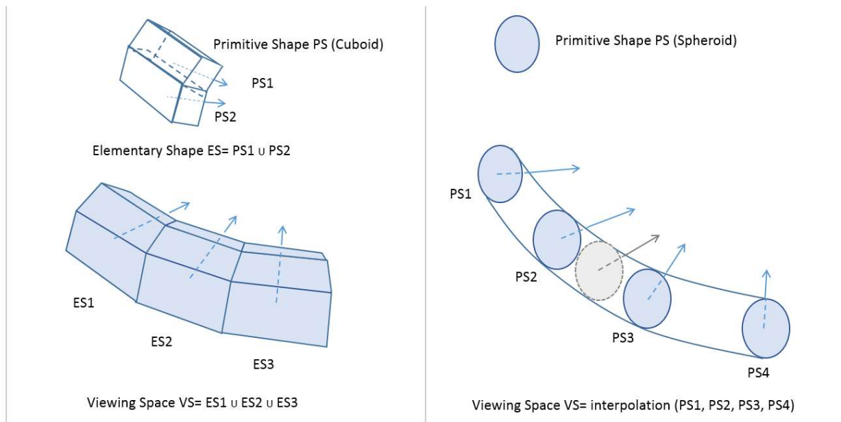
Figure 43: Illustration of VS creation with additive CSG (left) and interpolation (right)
