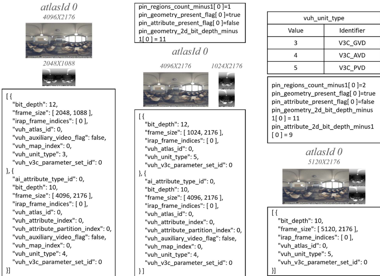
Figure 27: Geometry packing for MIV anchor – ClassroomVideo sequence at frame 0: MIV anchor (left), geometry packing (center), geometry packing + attribute bitstreams merging (right)
