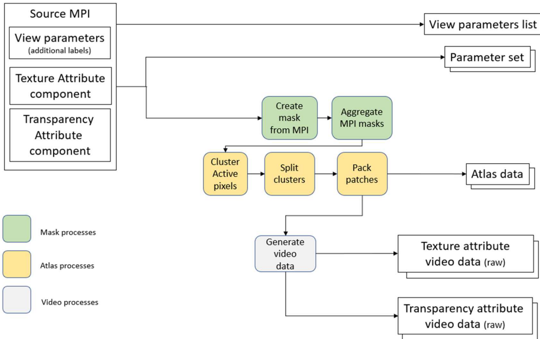
Figure 34: Top-level diagram of the TMIV MPI encoder
