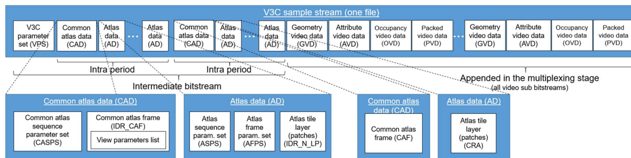
Figure 35: V3C sample stream with MIV extensions
