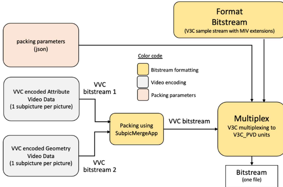
Figure 28: Encoding of texture and geometry components into one packed video sub-bitstream
