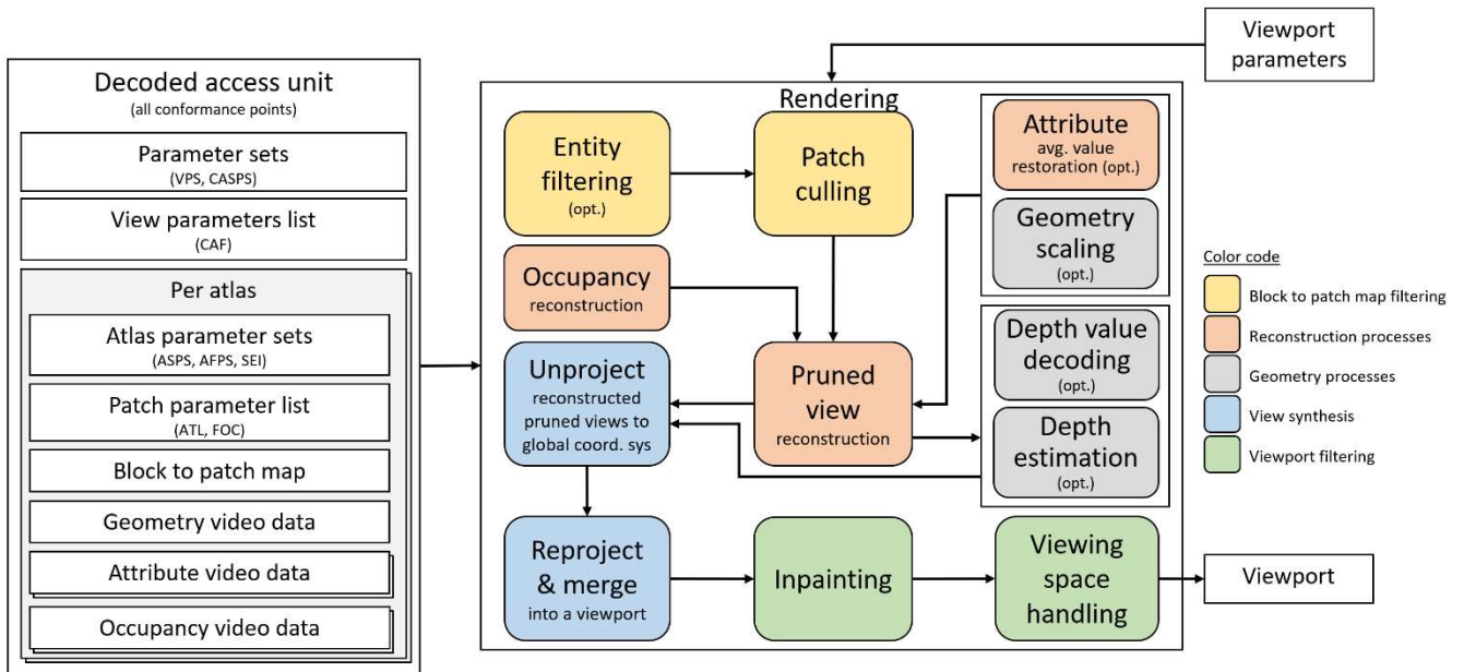
Figure 36: Process flow for the TMIV renderer
