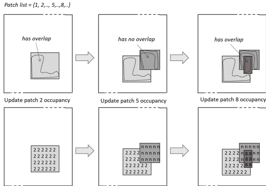
Figure 37. Occupancy map update in an ordered manner with patch culling
