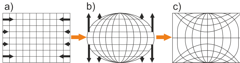
Figure 42: Fast reprojection of an equirectangular image (a) to transverse equirectangular image (c). Black arrows show direction of change of size of respective rows and columns of images
